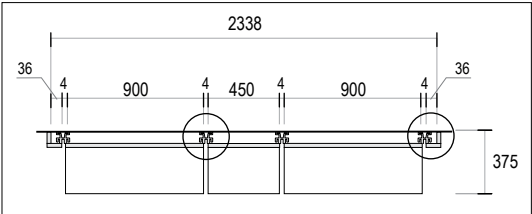
Larghezza visibile tra mensole 4 mm Visible width between shelves 4 mm Largeur visible entre étagères 4 mm
