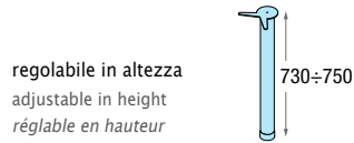
Gamba BOLD Leg / Pied
