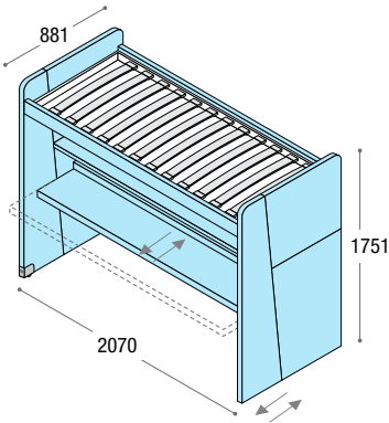
Chiuso Closed / Fermé
