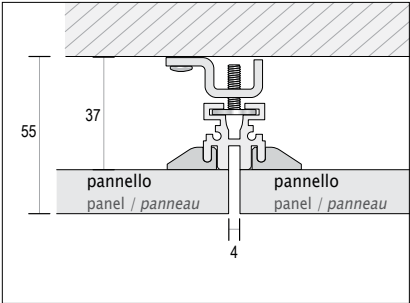
Cremagliera intermedia Central slotted rail / Crémaillère centrale
